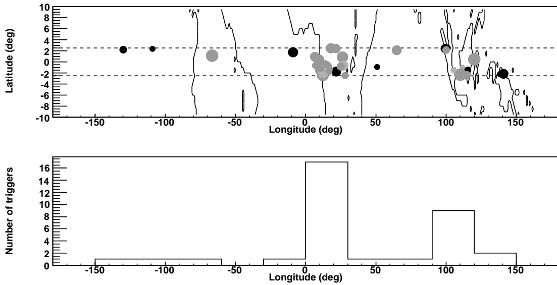
Figure 4. Geographical distribution of the selected triggers. Top panel: scatter plot of the geographical footprint of the AGILE satellite for the selected events. The radius of each dot is proportional to the number of counts, the color indicates the hardness ratio (the brightest the hardest) according to the data reported in Table 2. The dashed horizontal lines mark the maximum latitudes reached by AGILE. Bottom panel: longitude distribution of the sample.
