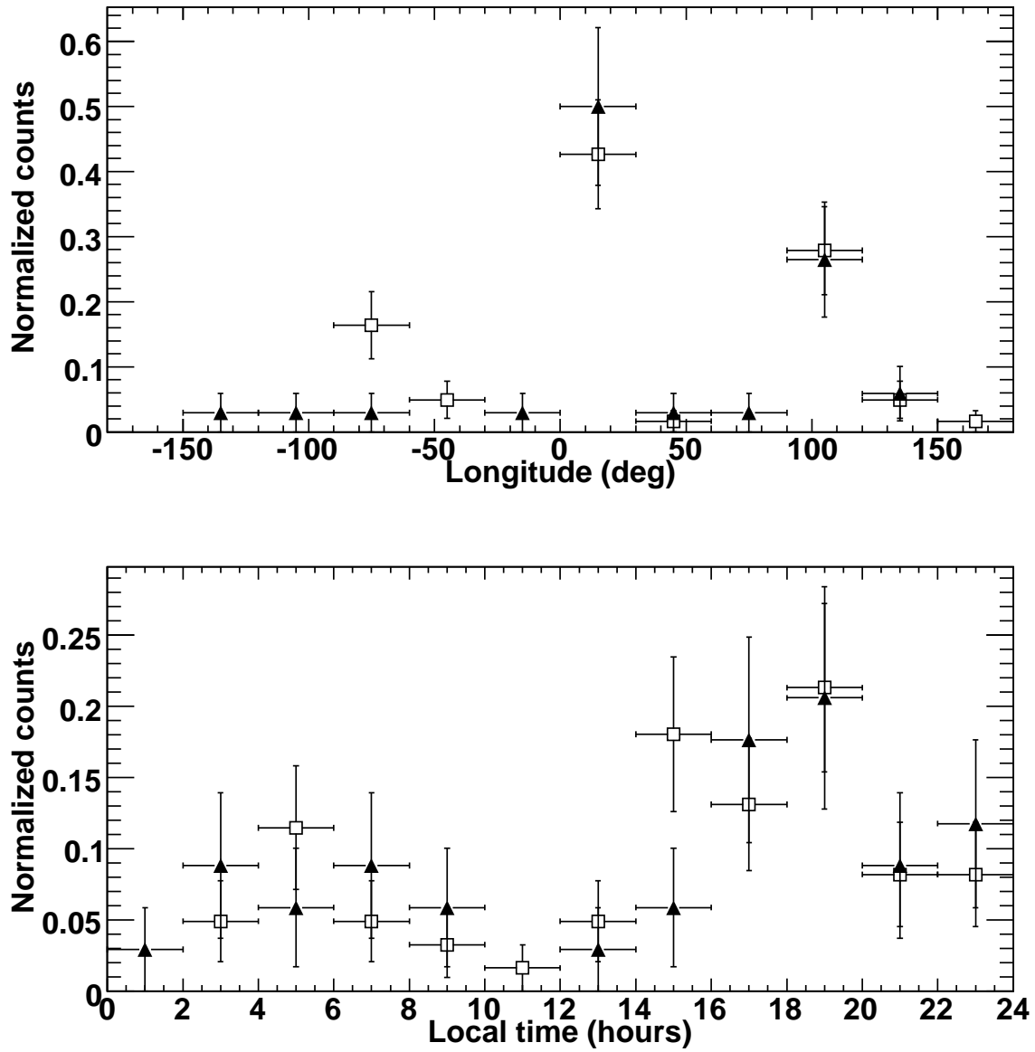
Figure 6. Geographic longitude (top panel) and local time (bottom panel) distributions for AGILE (filled triangles) and RHESSI (hollow squares) TGFs samples. The vertical axis error bars are one standard deviation assuming Poisson distribution.
