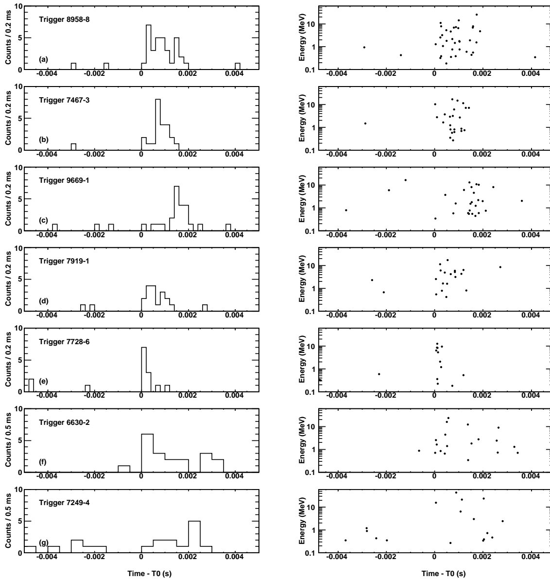
Figure 3. Light curves (left panels) and energy vs time plot (right panels) for several TGF candidates. Panels (a-c): the three brightest events. (d): the event with the largest hardness ratio. (e): the shortest event. (f): the longest duration event. (g): the event with the highest energy photon.
