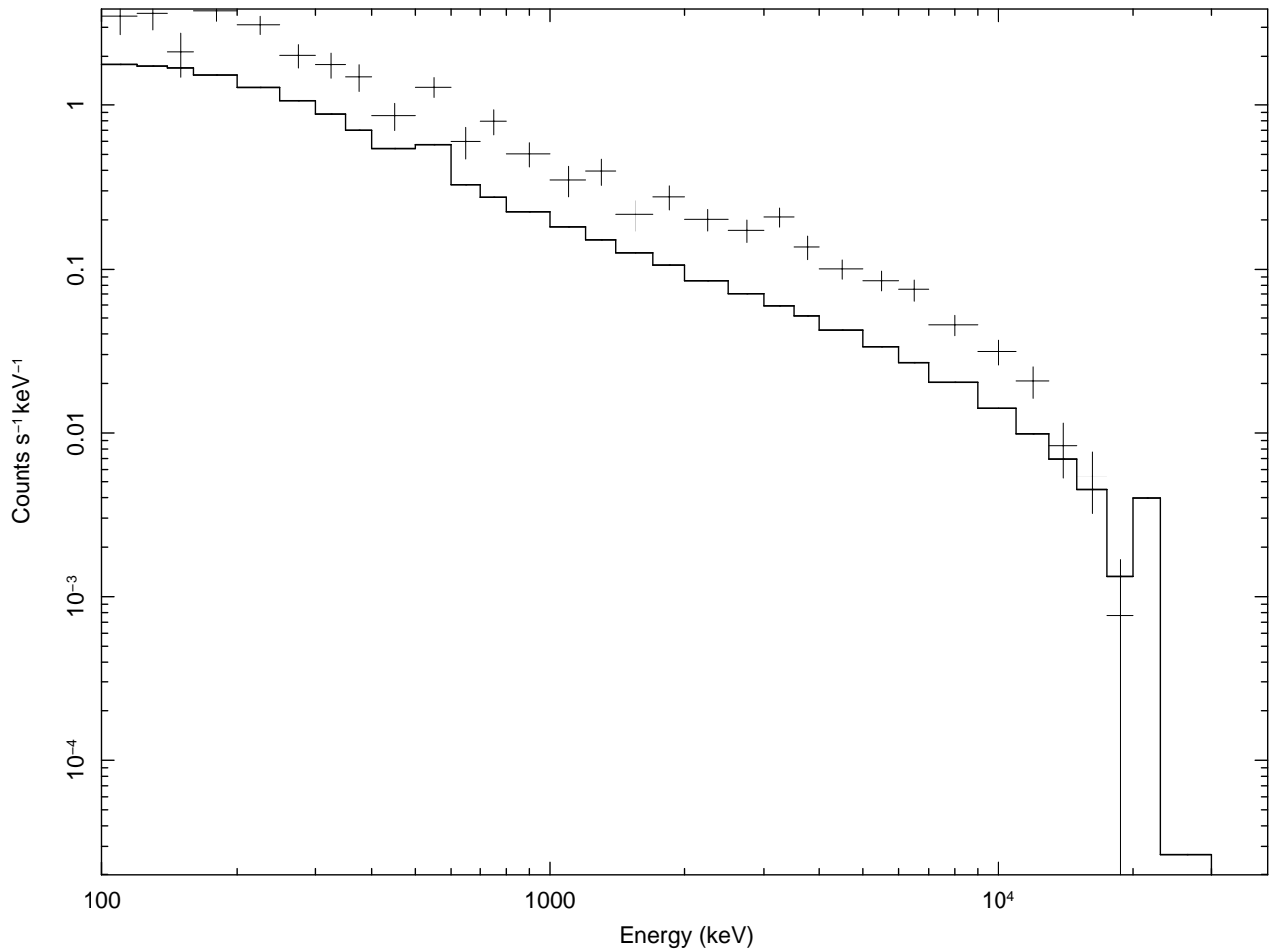
Figure 7. RHESSI experimental cumulative count spectrum for events triggered before 1 st January 2005 at latitudes lower than 2.5° in absolute value. Solid curve: MCAL best fit model convolved with the RHESSI response matrix.
