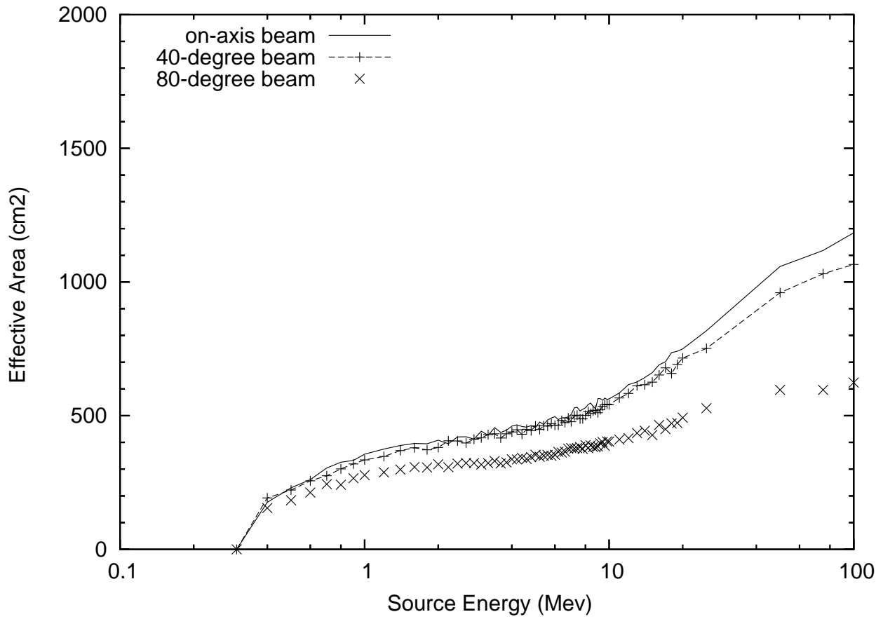
Figure 1. MCAL total effective area as a function of energy, from Labanti et al. [2009].
