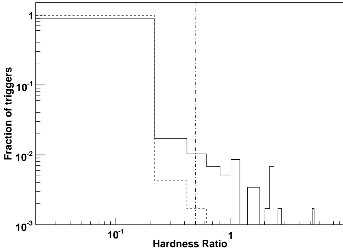
Figure 2. Normalized hardness ratio distribution for triggers of instrumental origin (dashed line) and for the other triggers (solid line). Only events with at least 10 counts have been selected. The vertical dot-dashed line marks the HR = 0.5 value.
