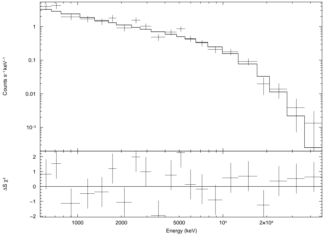
Figure 5. Top panel: cumulative background-subtracted count spectrum for the MCAL TGF sample. A cutoff powerlaw best fit model convolved with the instrumental response (see text for details) is superimposed on the data (solid line). Bottom panel: the residual distribution.
