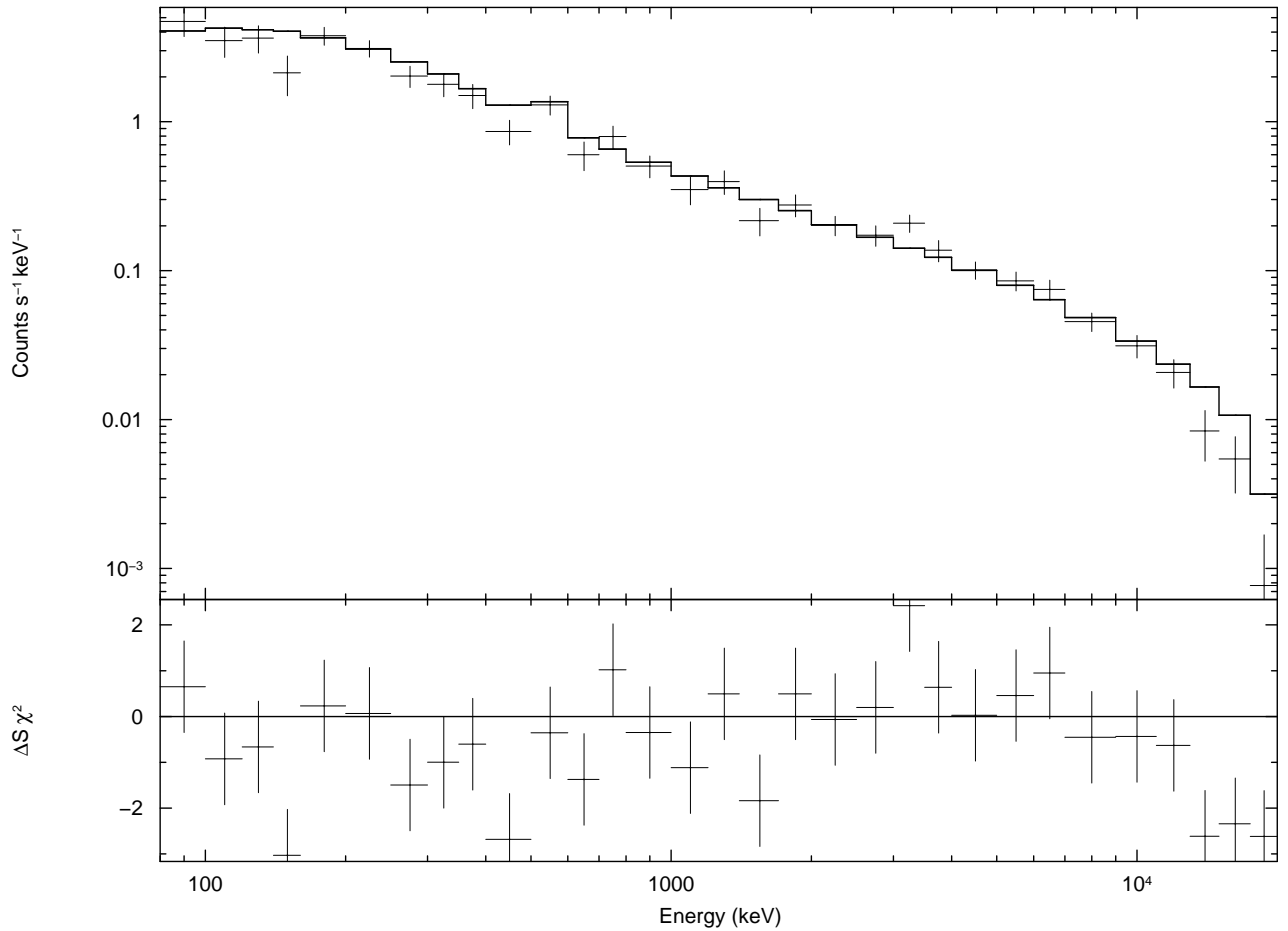
Figure 8. RHESSI experimental cumulative count spectrum for events triggered before 1 st January 2005 at latitudes lower than 2.5^\circ in absolute value. (top panel) Solid curve: the MCAL best fit model convolved with the RHESSI response matrix after the normalization factor is fit to RHESSI data (spectral parameters are kept constant). (bottom panel) The fit residuals.
